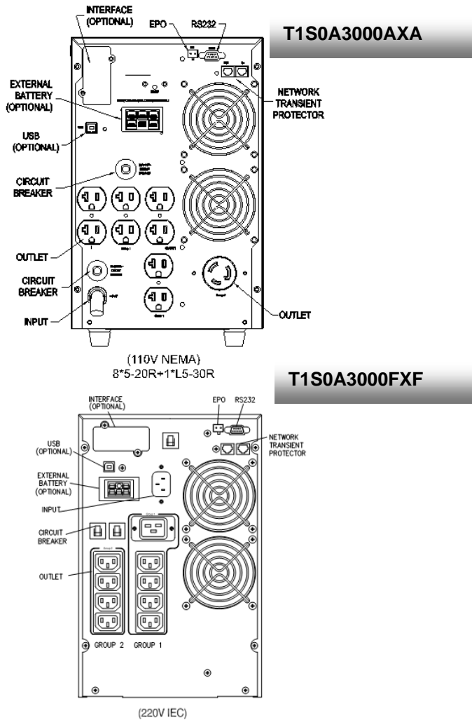
Figure 4 3000VA Tower Rear Panel View
