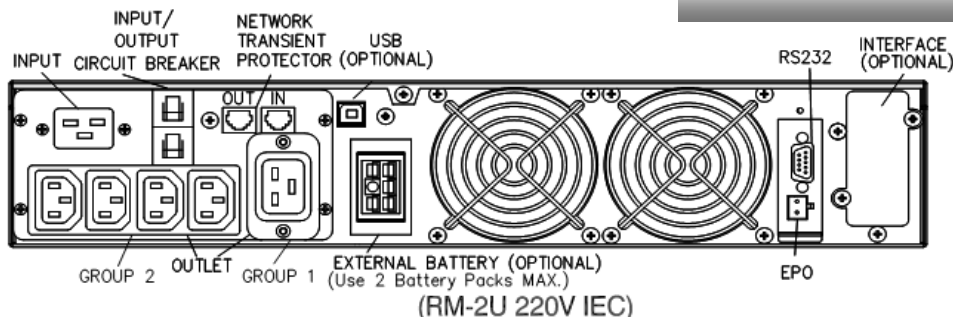
Figure 7 3000VA Rackmount Rear Panel View
