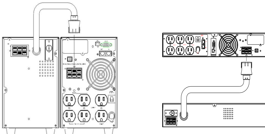
Figure 9 Connecting External Battery Cabinet
