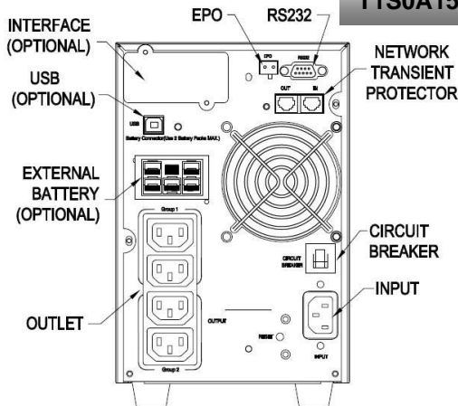
Figure 2 1000VA & 1500VA Tower Rear Panel View
