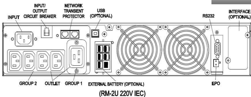
Figure 6 2000VA Rackmount Rear Panel View
