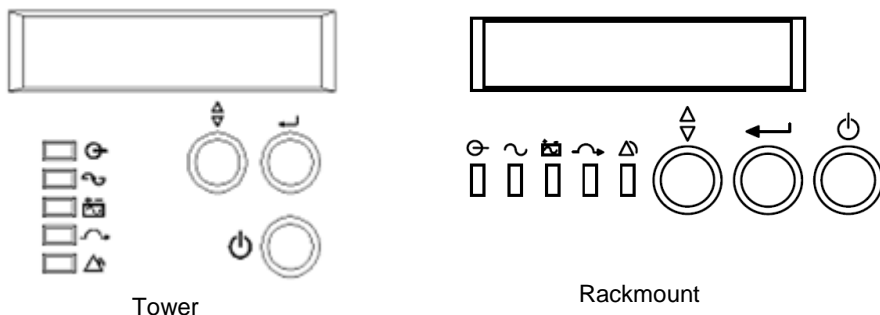
Figure 10 Control Panel Layout
