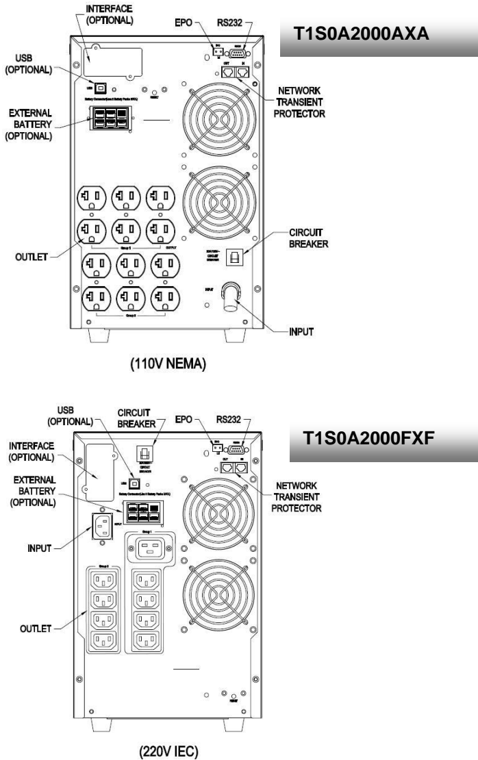
Figure 3 2000VA Tower Rear Panel View
