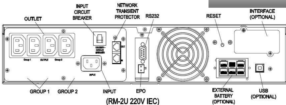
Figure 5 1000VA & 1500VA Rackmount Rear Panel View
